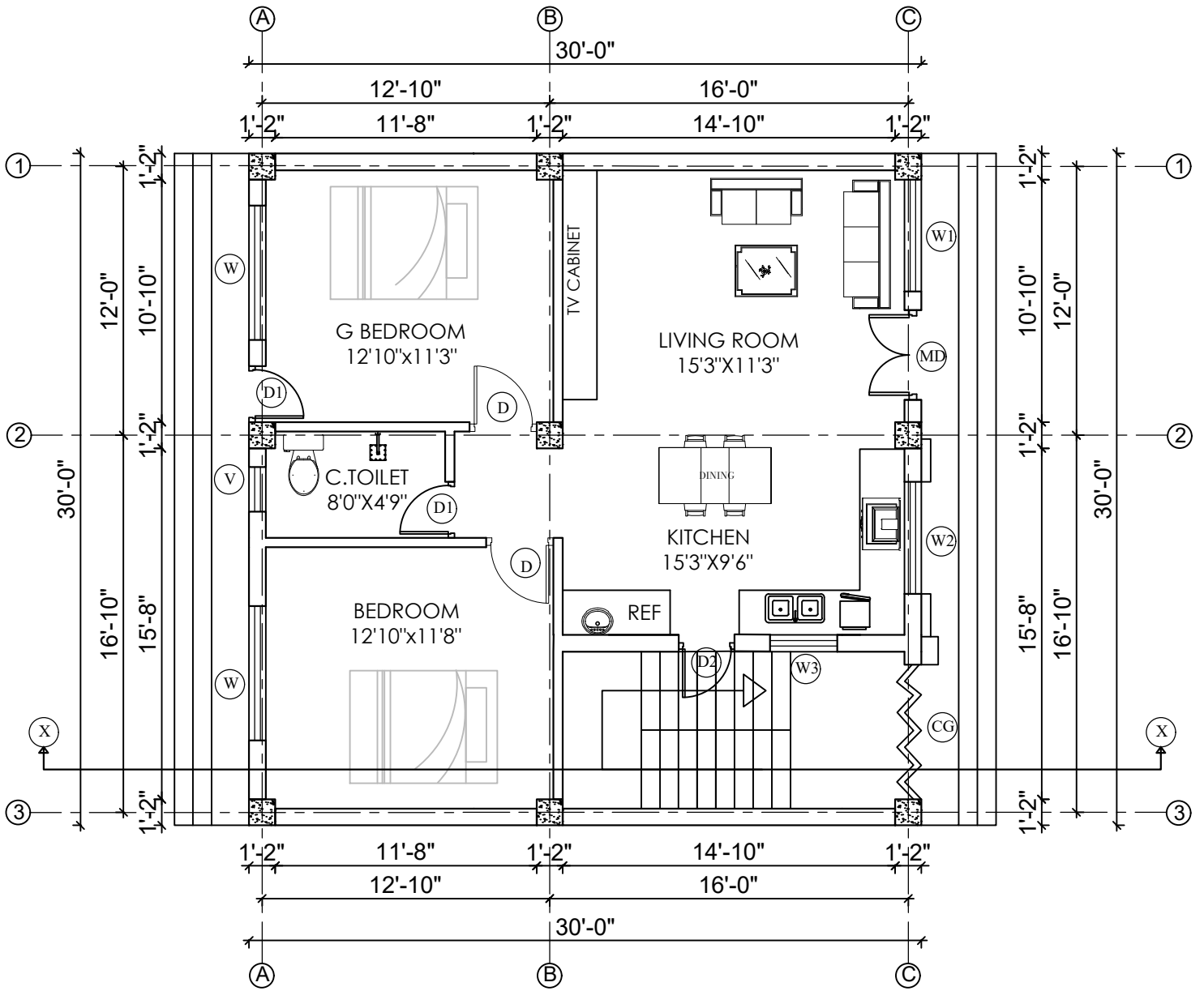
GROUND FLOOR PLAN : 900 SQ.FT
